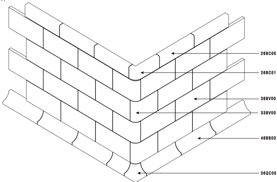
OUT-CORNER WITH BOX CAP & ELLIS COVE BASE
