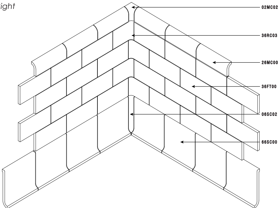
IN-CORNER WITH MUD CAP & SHOULDER COVE BASE
